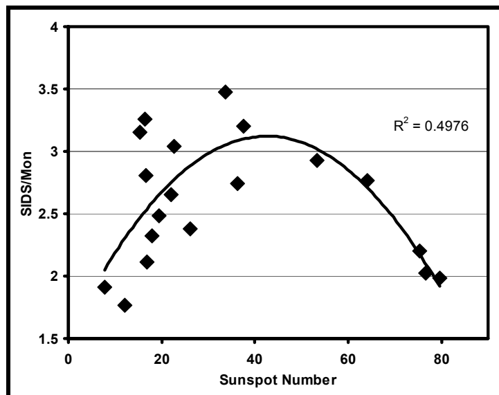
Figure 4: The 3-month running mean, seasonal and trend removed SIDS monthly rate and sunspot number during a transitional sunspot period, February 1984 to August 1985, “∩” curve trend, p < 0.001 .
