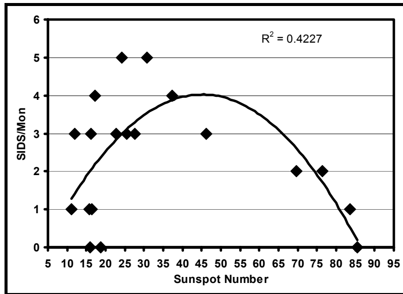
Figure 3: The raw SIDS monthly rates vs Sunspot Number during a transitional sunspot period a few years after sunspot maximum, February 1984 to August 1985. “∩” curve trend p < 0.005 .
