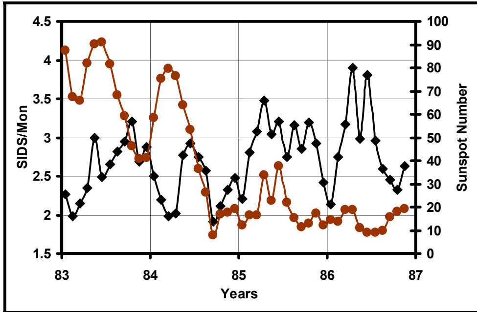
Figure 10: Time series of 3-month smoothed mean, seasonal and trend adjusted rates of SIDS (black) and sunspot number (red), for the period from January 1983 to November 1986.
