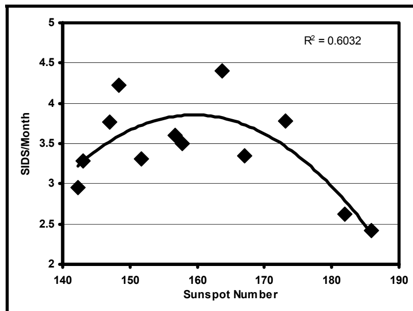
Figure 7: The 3-month running mean, seasonal and trend removed SIDS monthly rate and sunspot number during a high and declining sunspot period, August 1981 to April 1983, “ \cap ” curve trend, p < 0.0002 .
