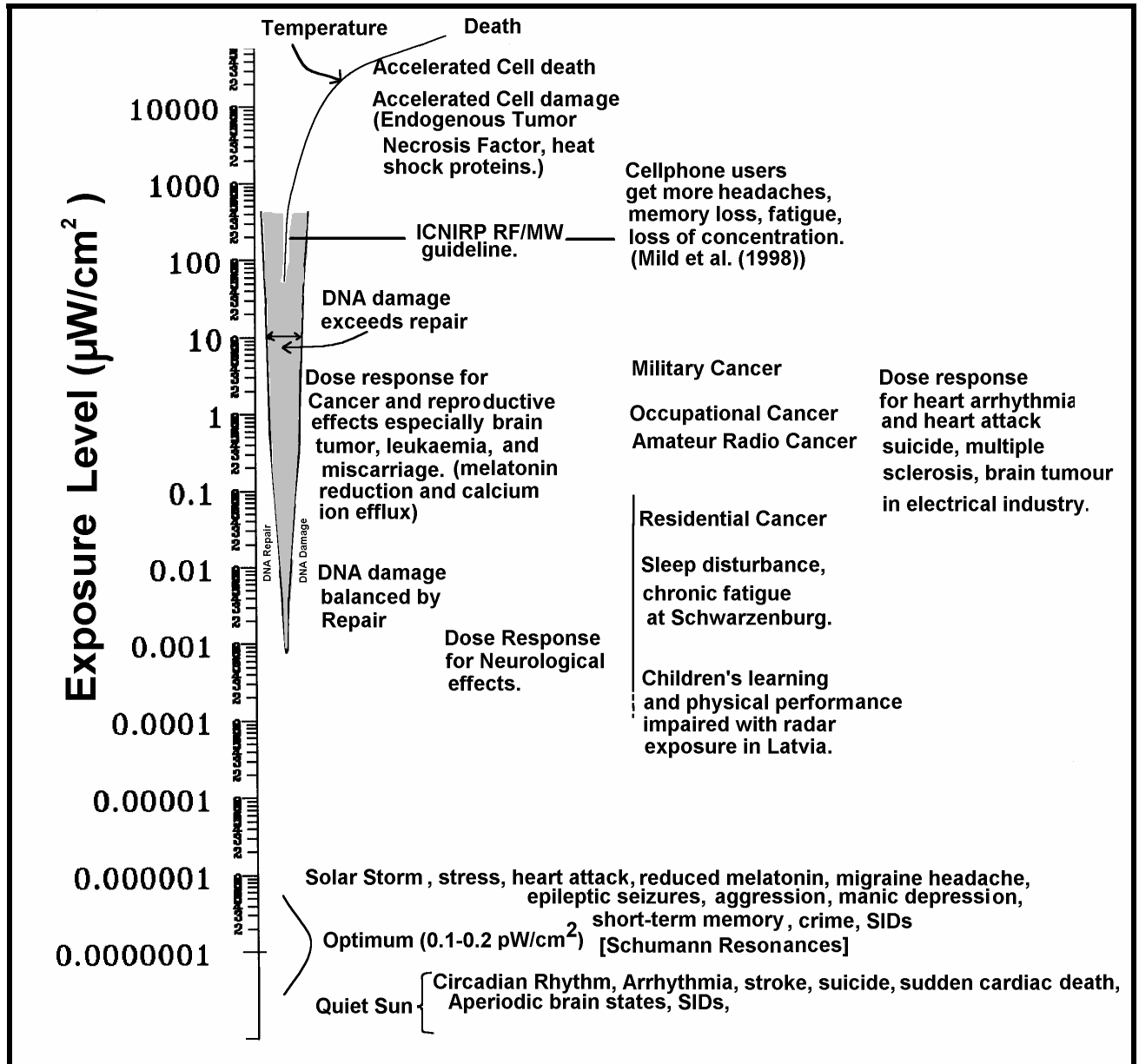
Figure 48: Summary of observed effects, and the mean levels of the exposure for human studies of exposure to electromagnetic radiation. All epidemiological studies occur below the ICNIRP and WHO guidelines.
