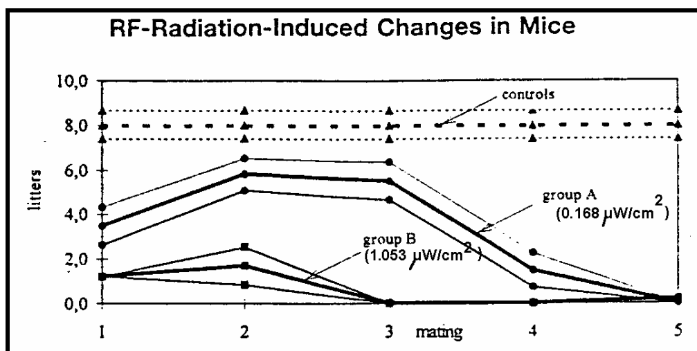
Figure 45: Reproductive rates in two groups of mice exposed to extremely low intensity radio signals, showing a dose response in the time taken to achieve full infertility of 3 matings for 1.053\mu\text{W}/\text{cm}^2 and 5 matings for 0.168\mu\text{W}/\text{cm}^2 .
