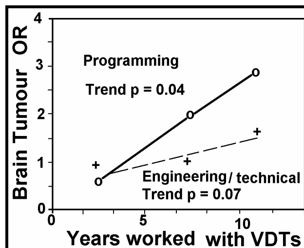
Figure 42: Dose-response increases in brain tumour from years of working with computers, Beall et al. (1997).
