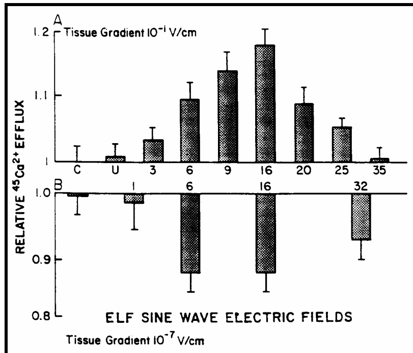
Figure 3: ELF induced calcium ion efflux in chick brain cells from (A) an ELF modulated 147 MHz signal and (B) an ELF signal, Bawin, Kaczmarek and Adey (1975).
