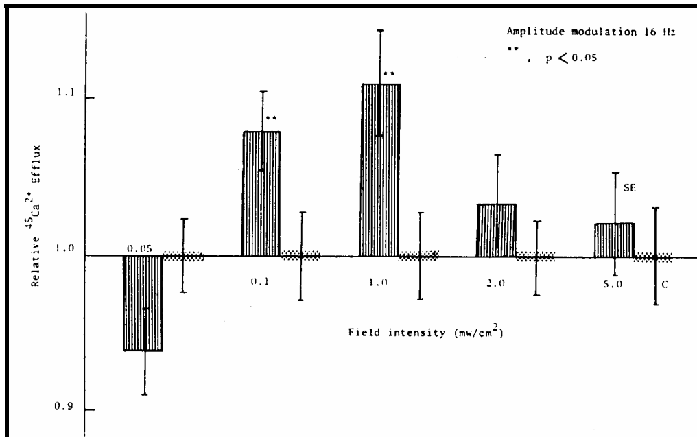
Figure 6: Effects of changing intensity of 450 MHz field, amplitude modulated at 16 Hz, on the efflux of calcium ions from chick cerebral hemispheres, Bawin, Sheppard and Adey (1978).
