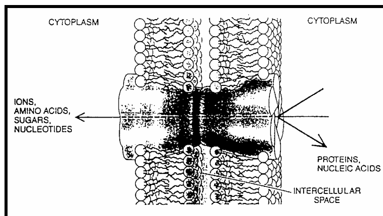
Figure 9: A Gap Junction structure, a six-element protein bridge that allows selective molecules to pass between cells as part of the cell-to-cell communication to coordinate cell regulation.
