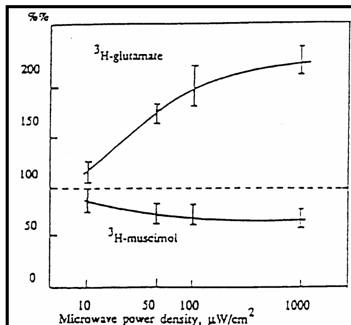
Figure 43: Exposure related alteration of GABA related molecules in rat brains exposed to 915 MHz microwaves, pulsed at 16 pps. Differences from controls are still significant at 10\mu\text{W}/\text{cm}^2 , Kolomytkin et al. (1995)
