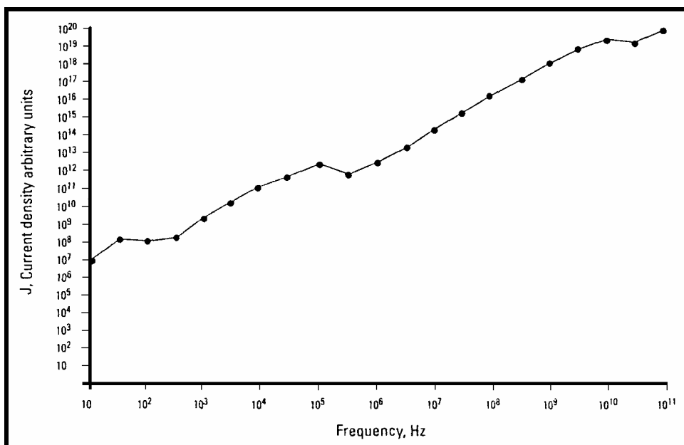
Figure 8: Capacitive current density in a toroid of human muscle tissue of unitary radius, to a unitary magnetic induction, Vignati and Giuliani (1997).
