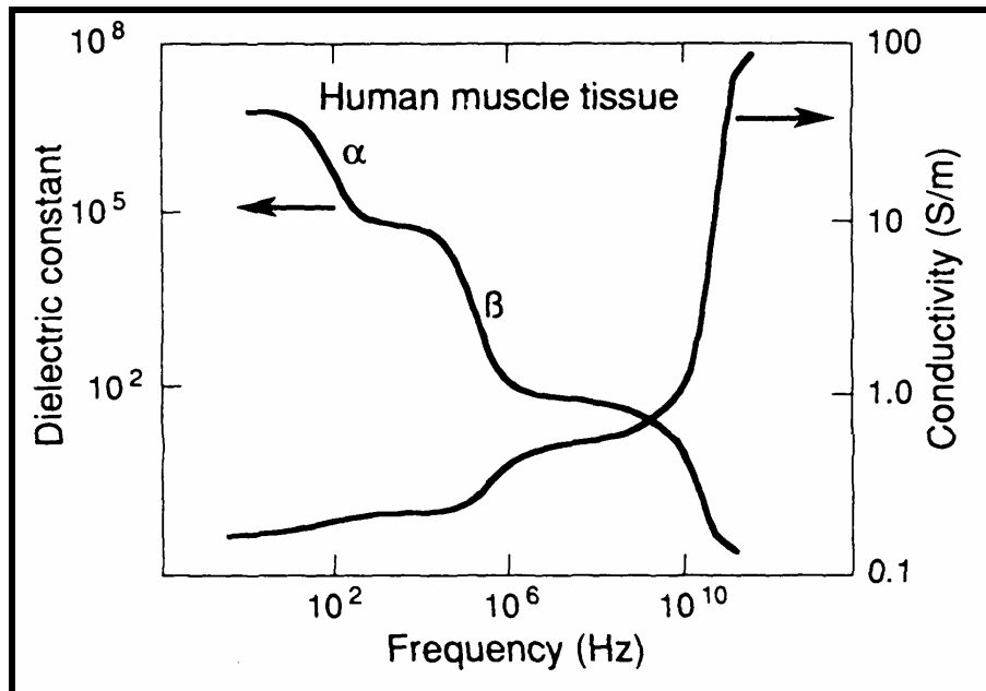
Figure 7: The dielectric constant and the conductivity for human muscle tissue as a function of the carrier frequency, From Schwan (1985) cited in WHO (1993).
