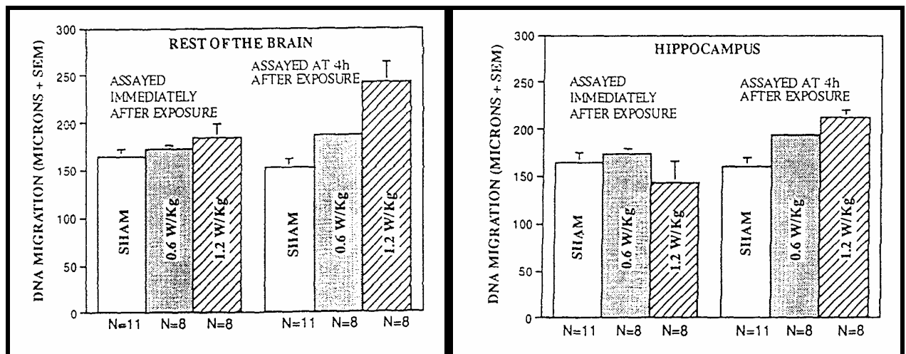
Figure 26: DNA single-strand breakage in cells from the rat brain and hippocampus, immediately after a 2 hr exposure to a whole body SAR of 0.6 and 1.2 W/kg to 2.45 GHz microwave radiation, pulsed at 500 pps. N is the number of rats studied. Lai and Singh (1995).
