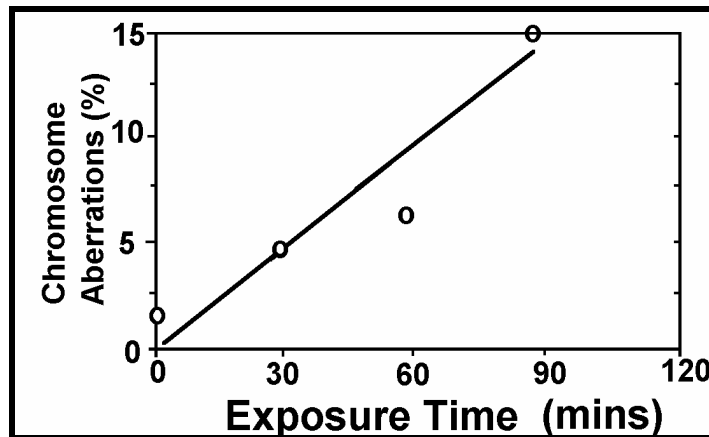
Figure 16: Chromosome aberrations in V79 Chinese hamster cells exposed to 7.7 GHz microwaves at 30 mW/cm 2 , Garaj-Vrhovac, Horvat and Koren (1991).
