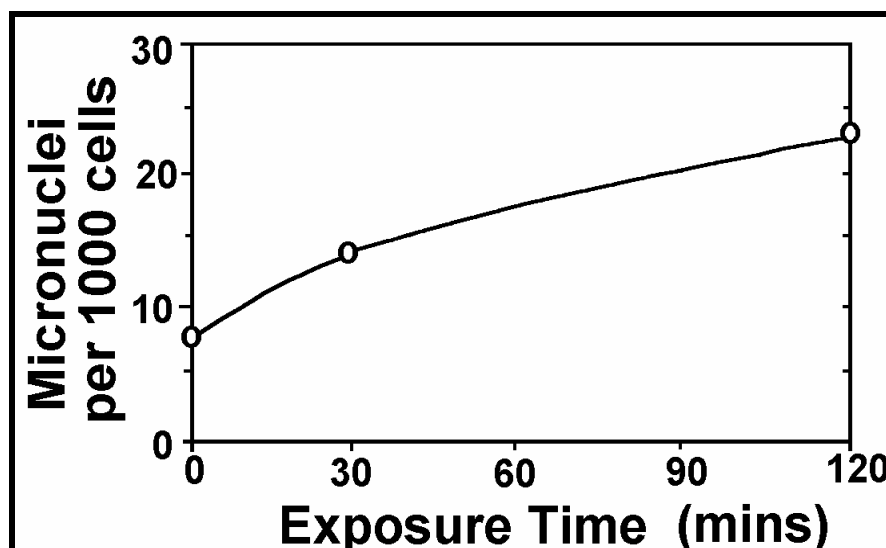
Figure 20: Micronuclei in microwave exposed human lymphocytes, the average of 4 donors, Maes et al. (1993). Exposure was to 75 W/kg, 2.45 GHz microwaves pulsed at 50 Hz, under controlled isothermal conditions
