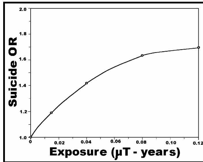
Figure 41: Dose response relationship of Suicide after recent monitored exposure to cumulative 50 Hz magnetic fields for men <50 years, adjusted for work, class, location and exposure to sunlight and solvents, Wijngaarden et al. (1999).
