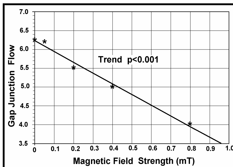
Figure 10: Gap junction flow as a function of 50 Hz magnetic field strength, Li et al. (1999).
