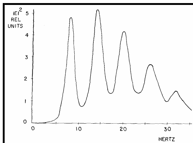
Figure 12: Daytime Schumann Resonance Spectrum, Polk (1982).
