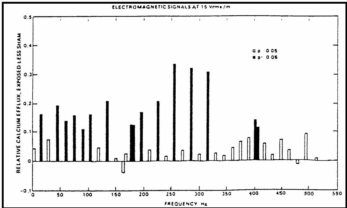
Figure 4: Effect of 15 Vrms/m electromagnetic fields on the efflux of calcium ions from chick brains as a function of modulation frequency, Blackman et al. (1988).
