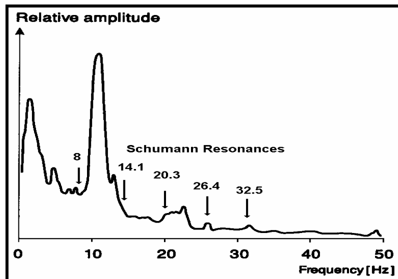
Figure 11: A typical EEG spectrum, with the Schumann Resonance peaks superimposed.
