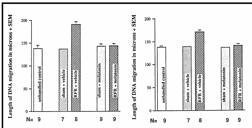
Figure 28: Effect of treatment with melatonin for RFR-induced increase in DNA single-strand (left) and double-strand (right) breaks in rats brain cells. Data was analysed using the one-way ANOVA, which showed a significant treatment effect ( p < 0.001 ) for both cases. "vehicle" involves injecting with the physiological saline without the active substance. Lai and Singh (1997)
