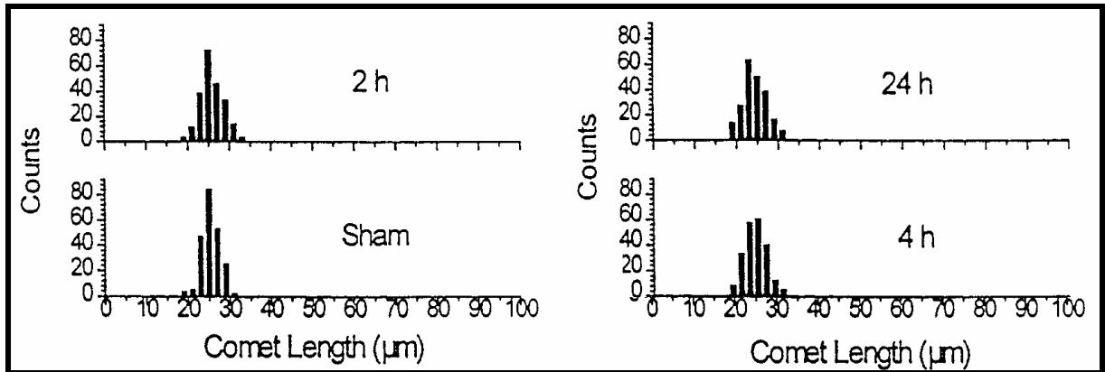
Figure 25: Frequency Distribution of Comet tail lengths for 2.45GHz exposed C3H10T1/2 cells, Malyapa et al. (1998), showing sham, 2 hr, 4 hr, and 24 hr exposure periods.
