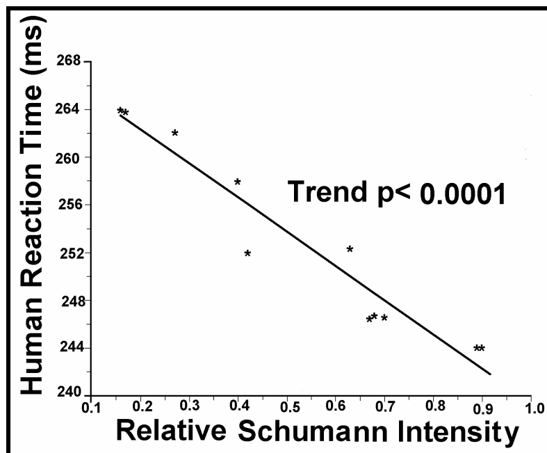
Figure 13: Human reaction times are causally correlated with natural variations in the Schumann Resonance Intensity, König (1974). The mean Schumann intensity (Relative Schumann Intensity =0.5) is 0.65mV/m or 0.1pW/cm 2 . The range is 0.2 to 1.2 mV/m (0.01 to 0.4pW/cm 2 ).
