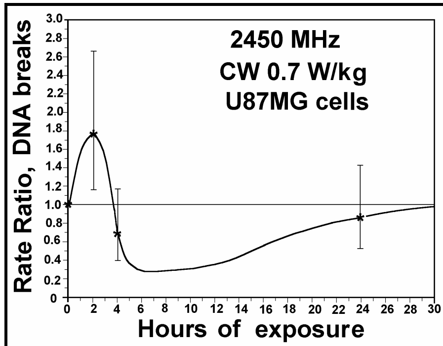
Figure 25a: The time sequence of DNA damage and enhanced repair for Figure 5 in Malyapa et al. (1997).
