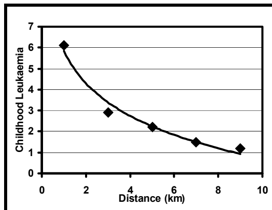
Figure 35: Cumulative childhood leukaemia near the Vatican Rome Radio Station with an exponential fitted trend line, R^2=0.9756 , p = 0.002 , Michelozzi et al. (2002).
