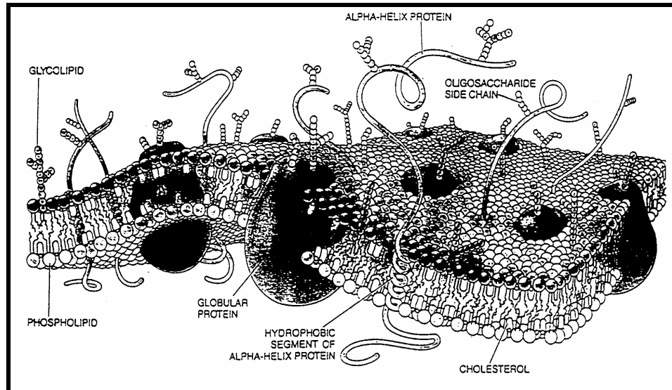
Figure 1: A schematic diagram of the cell membrane, showing the alpha helix of the signal transduction apparatus, with its "Y" shaped receptors on the alpha helix protein.
