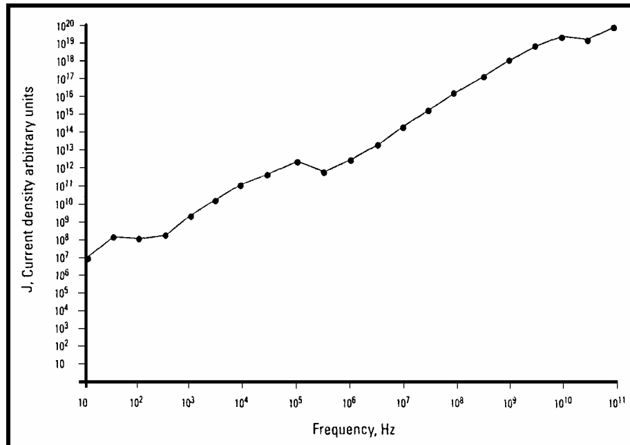
Figure 2: Induced tissue current from a unit applied field, as a function of the carrier frequency, Vignati and Giuliani (1997).
