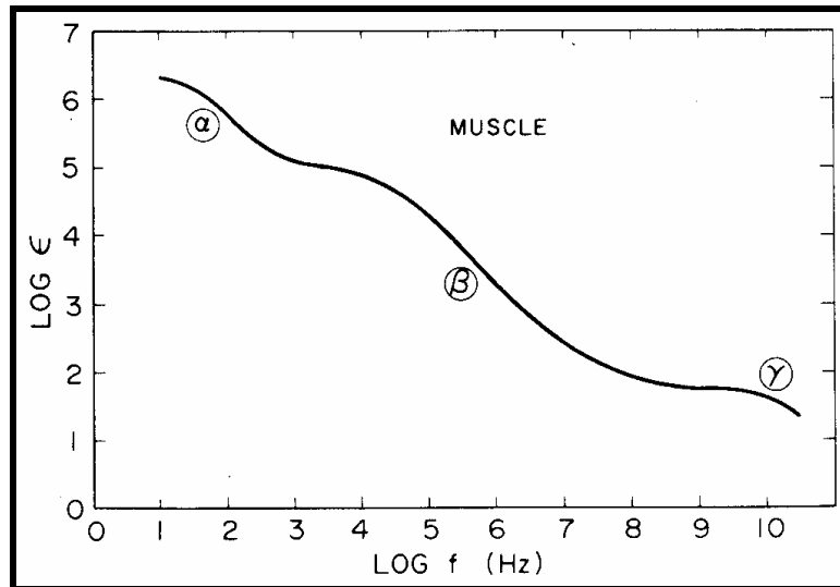
Figure 1: The dielectric constant of muscle as a function of frequency, Schwan and Foster (1980).
